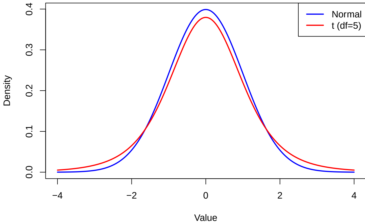
t-distribution vs Normal Distribution (df=5)
